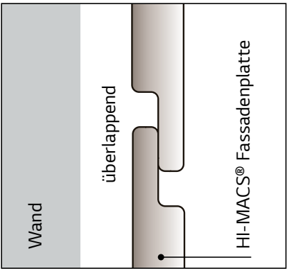
Überlappende Paneele
